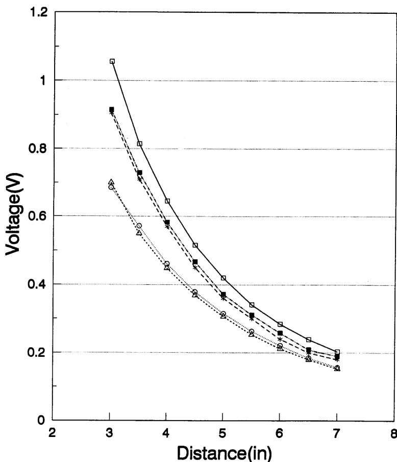
Fig. 1 Voltage detected by receiver as a function of distance between transmitter and receiver. □: no shielding material; Δ: steel mesh; ○ concrete with paper clips, cured horizontally; *: concrete with paper clips, cured vertically; ■ plain concrete. The voltage scatter was \pm 0.7\% for each data point in the case of concrete with paper clips, cured horizontally, and in the case of plain concrete. The voltage scatter was \pm 7\% for each data point in the case of concrete with paper clips, cured vertically. The voltage scatter was \pm 0.4\% for each data point in the case of steel mesh.
